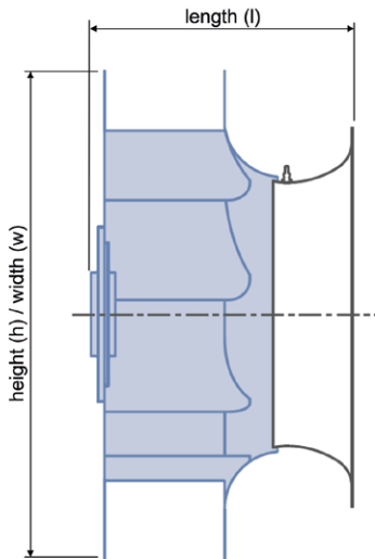
Figure 32 Dimensions for impellers
