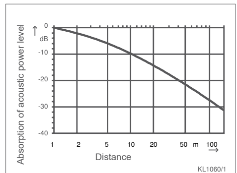
Fig. IV: Absorption of the acoustic pressure level
