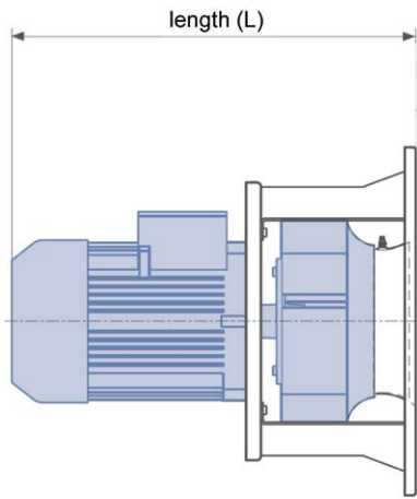
Figure 33 Dimensions of GR fans
