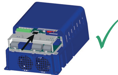
Memory card in the X-MMC card slot of ZAdyn4C 011-032
